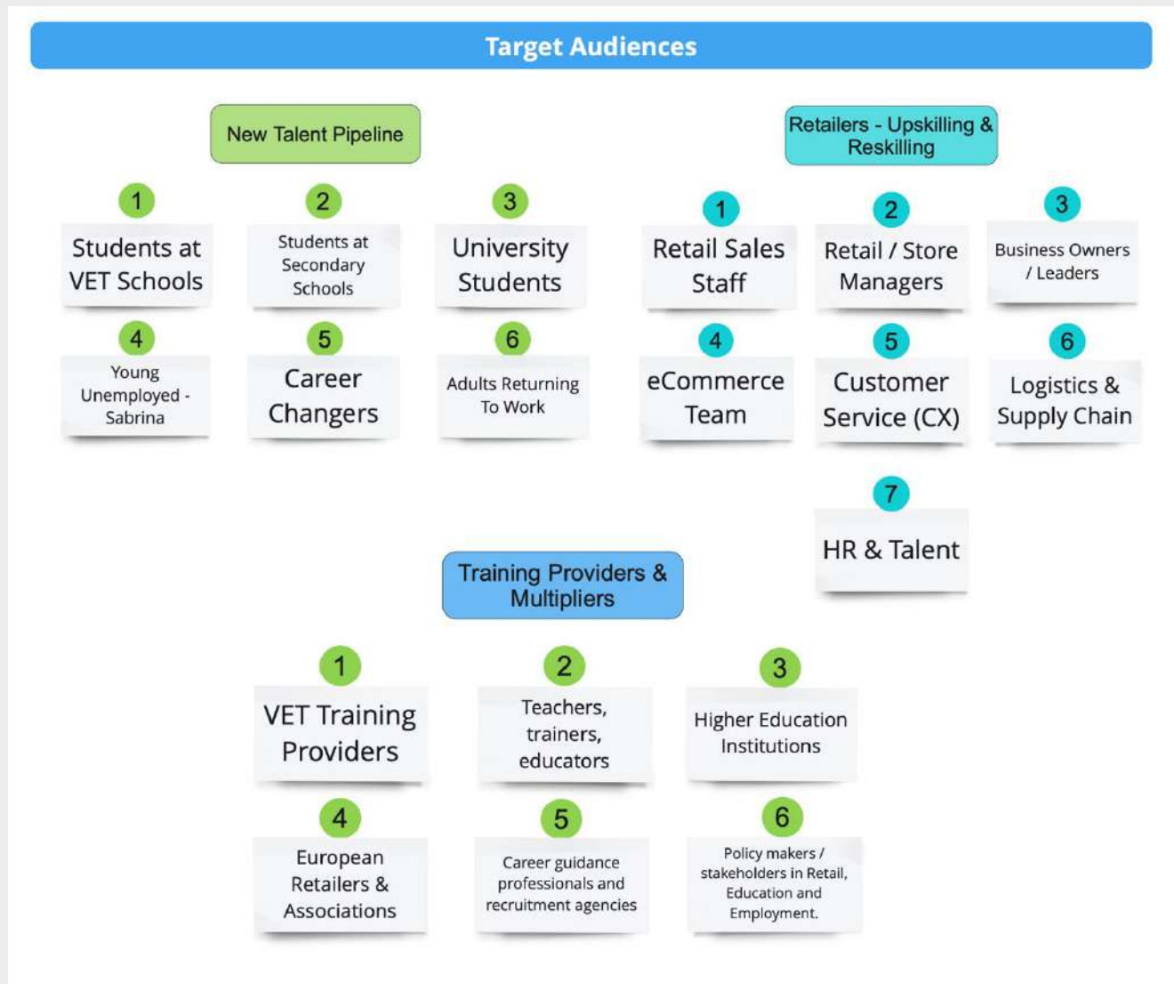
Figure 11 Target Audiences
